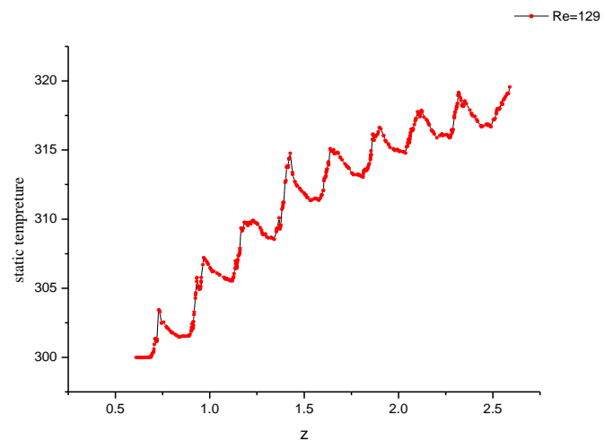
Fig. 7- Static temperature profile
