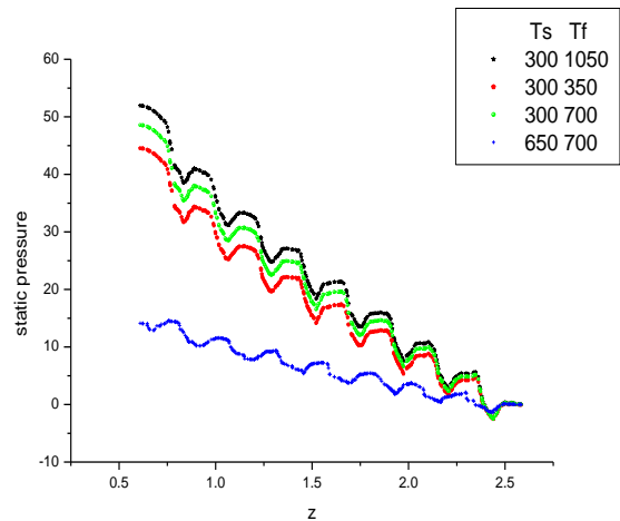
Fig. 10- Static pressure profiles.
