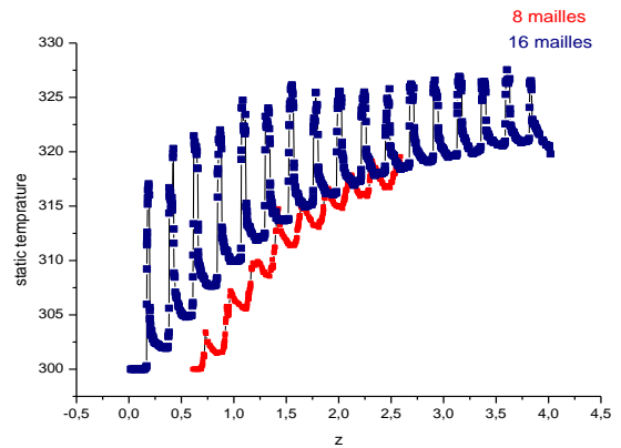
Fig. 14- Profile of temperature of tow thickness
