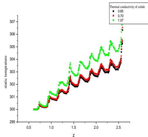
Fig 15-fluid temperature distributions for various solid thermal conductivities
